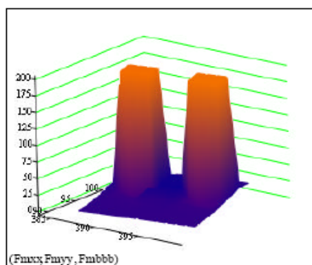
Figure 1: Distribution of magnetic field within the LVPS location window with max field distortion from ferrites - units in Gauss.
