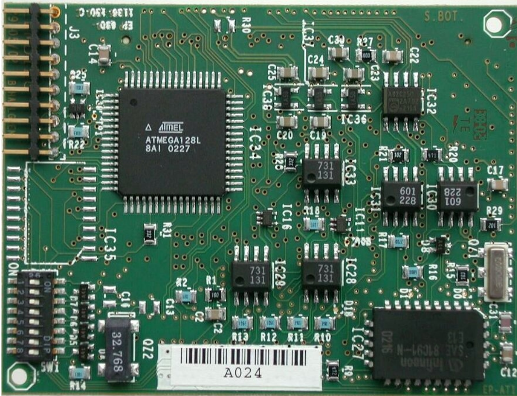
This is the back side of the ELMB128 ANALOG version with ADC
